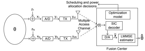
Fig. 1. WSN model for estimating the random signal \theta . Each sensor i transmits y_{d,i} , the digitized and modulated version of the analog sample. Simultaneously transmitting sensors are decoded by the SIC decoder.
