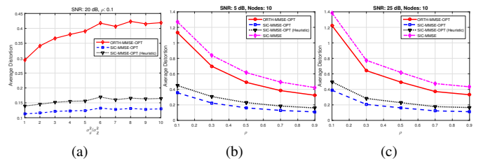
Fig. 4. The effect of the ratio \sigma_\theta^2/\sigma_z^2 (with \sigma_z^2 = 1 ) and \rho on average distortion.
